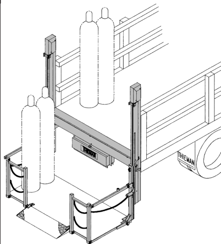
Platform in Loading/Unloading Position
