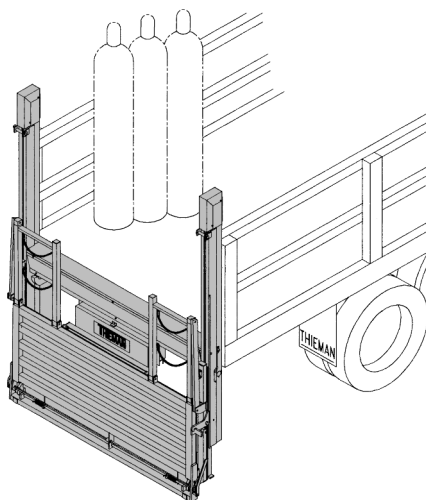
Platform in Docking Position
