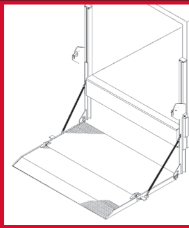
Platform in loading position
